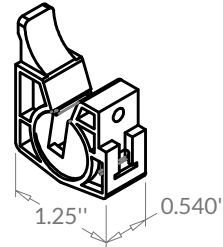
Nylon Shoe without break pin 1/2" RH white G1-32-SN1RH-01
