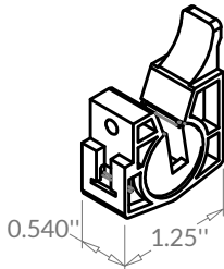
Reinforced Nylon Shoe without break pin 1/2" LH gray G1-32-SN1LH-07
