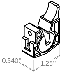
Nylon Shoe without break pin 1/2" LH white G1-32-SN1LH-01
