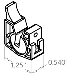
Reinforced Nylon Shoe without break pin 1/2" RH gray G1-32-SN1RH-07
