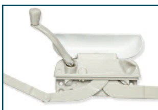
ECLIPSE double bras dual arm
